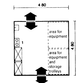
⑨ Supplies lobby
